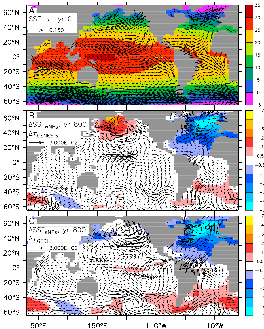
Figure 8. (a) Annual mean sea surface temperature ( ^{\circ}\text{C} ) of the control simulation at year 0, (b) stadial anomalies at year 800 for model version wNPs (without GENESIS wind stress anomalies), and (c) sNPs plus GFDL wind. Arrows show wind stress (Pa) for the control run (Figure 8a) and anomalies as obtained from the GENESIS model (Figure 8b) forced with the SST anomalies shown in (Figure 8b) and anomalies from the GFDL model (Figure 8c). Note that the length scale for the wind stress anomaly (indicated by the arrow in the top left corner) in Figures 8b and 8c is only 20% of that in Figure 8a.
