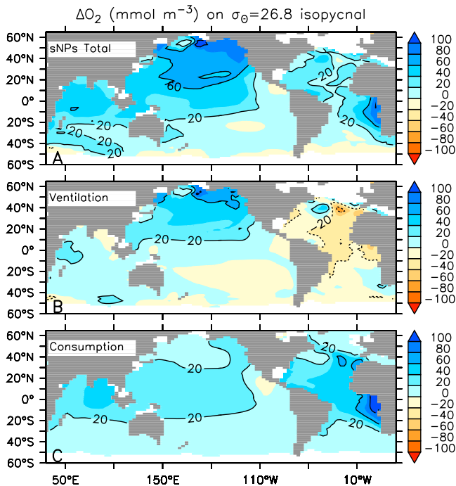
Figure 6. Oxygen anomaly on \sigma_\theta = 26.8 isopycnal surface at model year 800 as in Figure 2d. (a) Total anomaly (same as Figure 2d). (b) Anomaly due to ventilation changes only (experiment with constant interior oxygen sinks). (c) Anomaly due to consumption changes only (values of Figure 6a minus values of Figure 6b).
