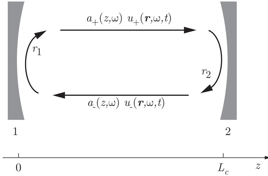
Figure 4.1: Cavity effects in a laser oscillator.
