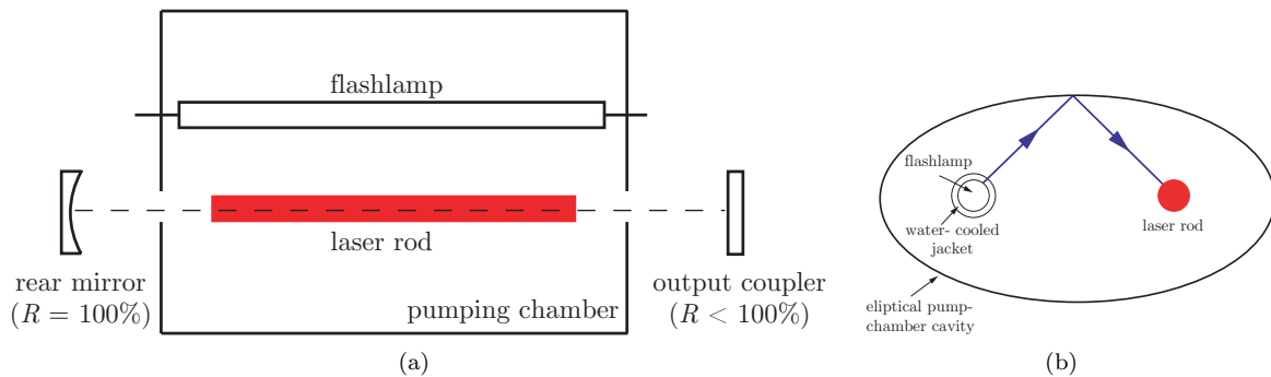
Figure 5.4: Schematic diagram showing: (a) the general layout of a flashlamp-pumped solid-state laser; (b) use of an elliptical pumping chamber to increase the efficiency with which flashlamp radiation is coupled into the laser rod.
