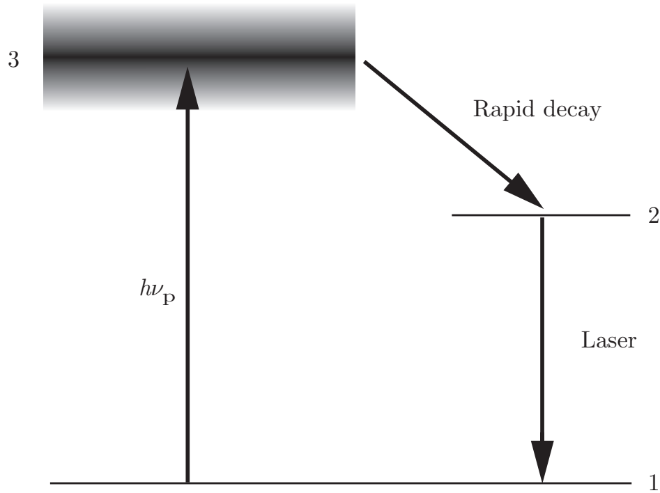
Figure 5.7: Simplified energy level diagram for calculation of the threshold pump energy in a three-level laser.
