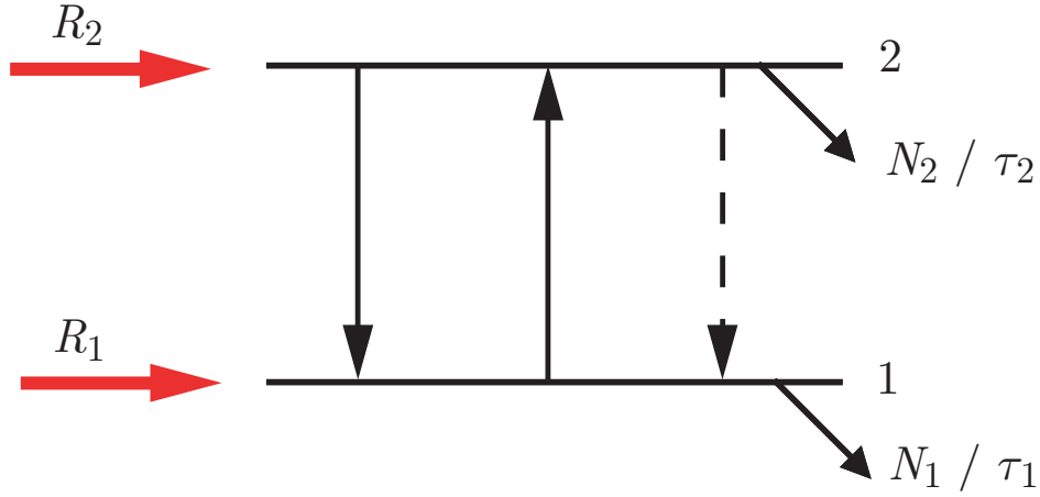
Figure 3.2: Processes affecting the upper and lower laser levels in a laser operating under steady-state conditions in the presence of an intense radiation beam.
