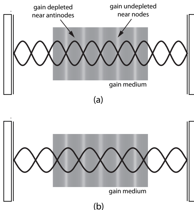
Figure 4.3: Spatial hole-burning in a homogeneously broadened steady-state laser oscillator. In (a) the standing wave of an oscillating mode causes the gain to be depleted where the intensity is high. However, the gain is unaffected near the nodes of the standing wave since the intensity in these regions is low. This can allow other cavity modes — which will have a different frequency and hence different locations for the nodes and antinodes in its standing wave pattern — to feed off the regions of unused gain, as shown in (b).
