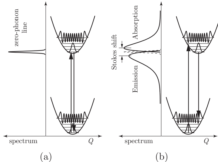
Figure 5.5: Transitions between electronic levels: (a) when the equilibrium configuration co-ordinate is essentially the same for the upper and lower electronic levels; (b) when the equilibrium configuration coordinates are different for the two levels, causing the potential curves to be displaced. Vibrational wave functions are illustrated schematically for the lowest vibrational level and an excited vibrational level. In (b) the position of the zero-phonon line is shown by the dotted curve.
