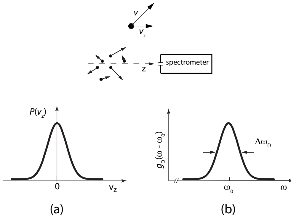
Figure 2.4: The formation of an inhomogeneously broadened spectral line by Doppler-broadened gas atoms. Radiation emitted by the atoms in the z -direction is detected by the spectrometer. The distribution of atomic velocities in the z -direction (a) leads, via the Doppler effect, to a distribution of frequencies measured by the spectrometer, and hence broadening of the spectral line (b).
