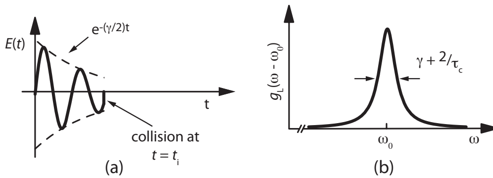
Figure 2.3: A simple model of collision broadening. A damped oscillating dipole is subject to a collision, leading to the electric field shown in (a). When averaged over the distribution of collision times, this gives rise to a frequency spectrum with a Lorentzian profile (b).
