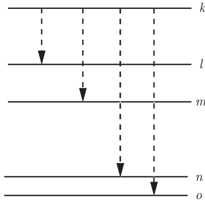
Figure 2.2: Radiative decay of an excited level k to lower levels \dots l, m, n \dots
