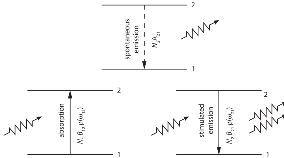
Figure 1.1: Illustration of the interaction of radiation with two levels of an atom by spontaneous emission, absorption, and stimulated emission. For each process the transition rates are given in terms of the Einstein coefficients and the number densities N_2 and N_1 of atoms in the upper and lower levels. The photons have energy \hbar\omega_{21} and the figure should be read from left to right. For example, in the case of stimulated emission an incident photon of energy \hbar\omega_{21} stimulates an excited atom to make a transition to the lower level, emitting a second photon in the process.
