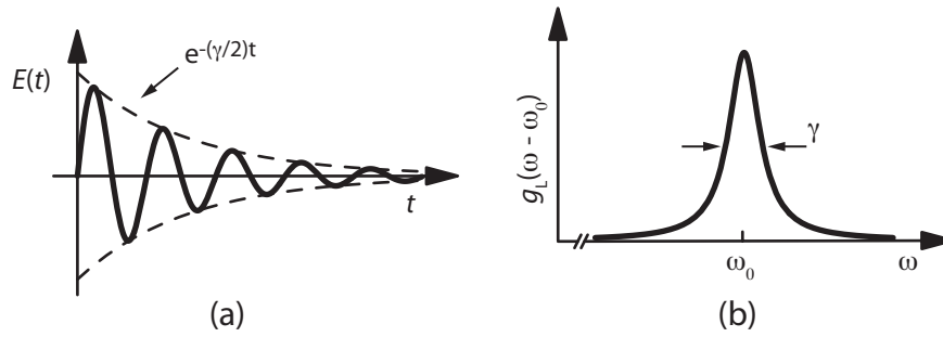
Figure 2.1: Illustrating how a damped oscillating electric field from a damped oscillating dipole (a) gives rise to a frequency spectrum with a Lorentzian profile (b).
