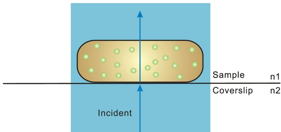
Epifluorescence
