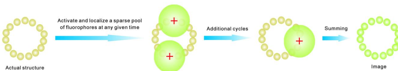
(B) PALM/STORM
